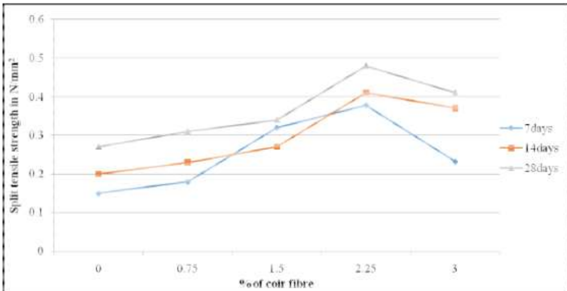
Figure 5 Split tensile strength
