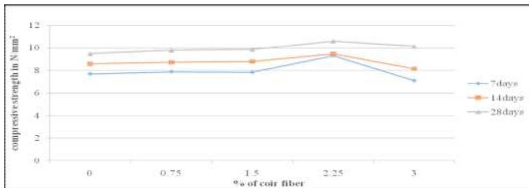
Figure 4 Compressive strength
