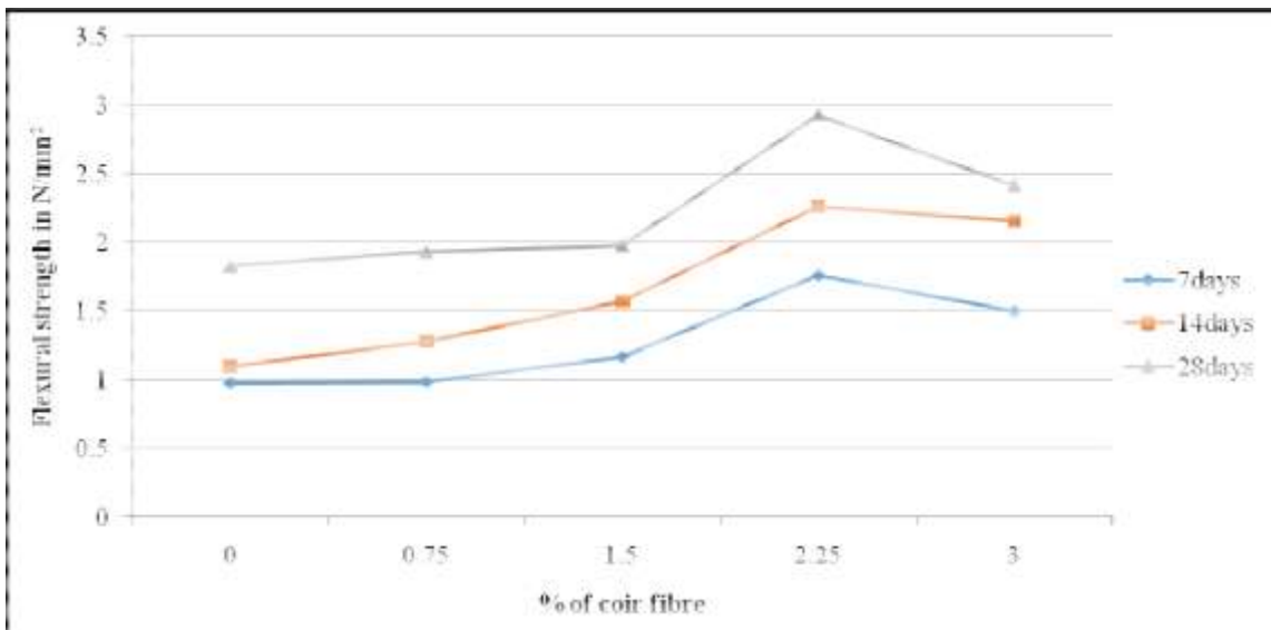
Figure 6 Flexural strength
